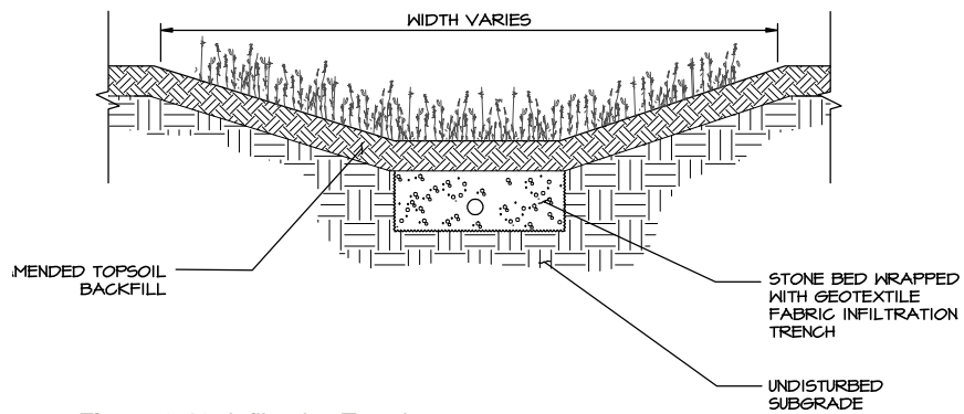
Figure 3-19: Infiltration Trench
