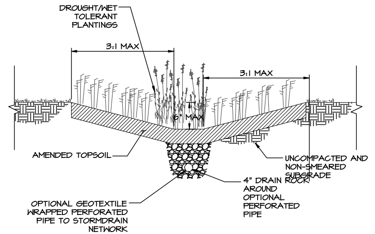
Figure 3-18 : Vegetated Swale
