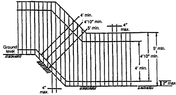
FIGURE 31B-4 PERPENDICULAR FENCING DIMENSIONS ON SLOPING GROUND
