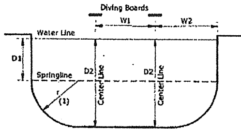
Transverse Section Deep End
